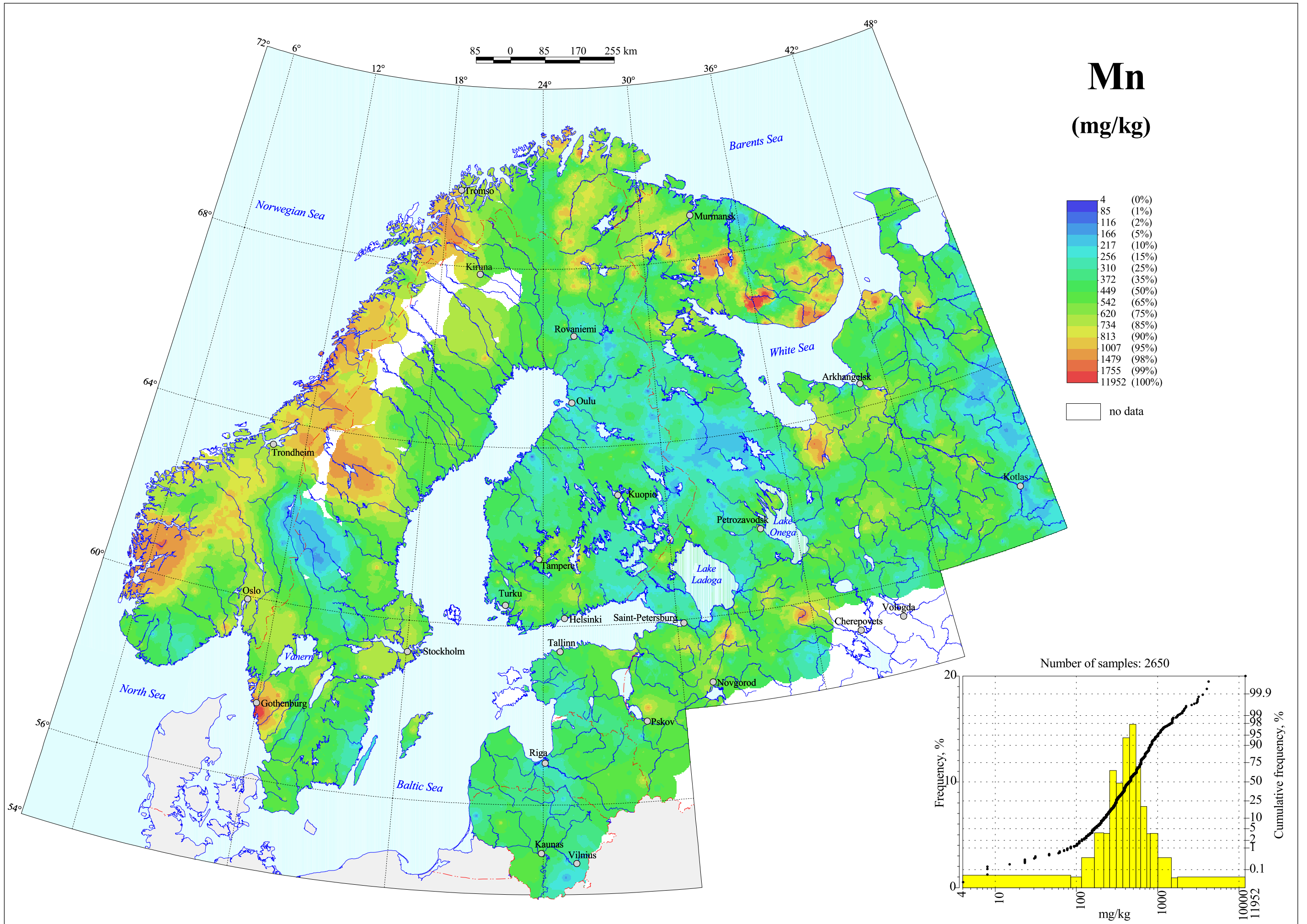
Manganese in C-horizon, Grain Size <2 mm, Total Content
